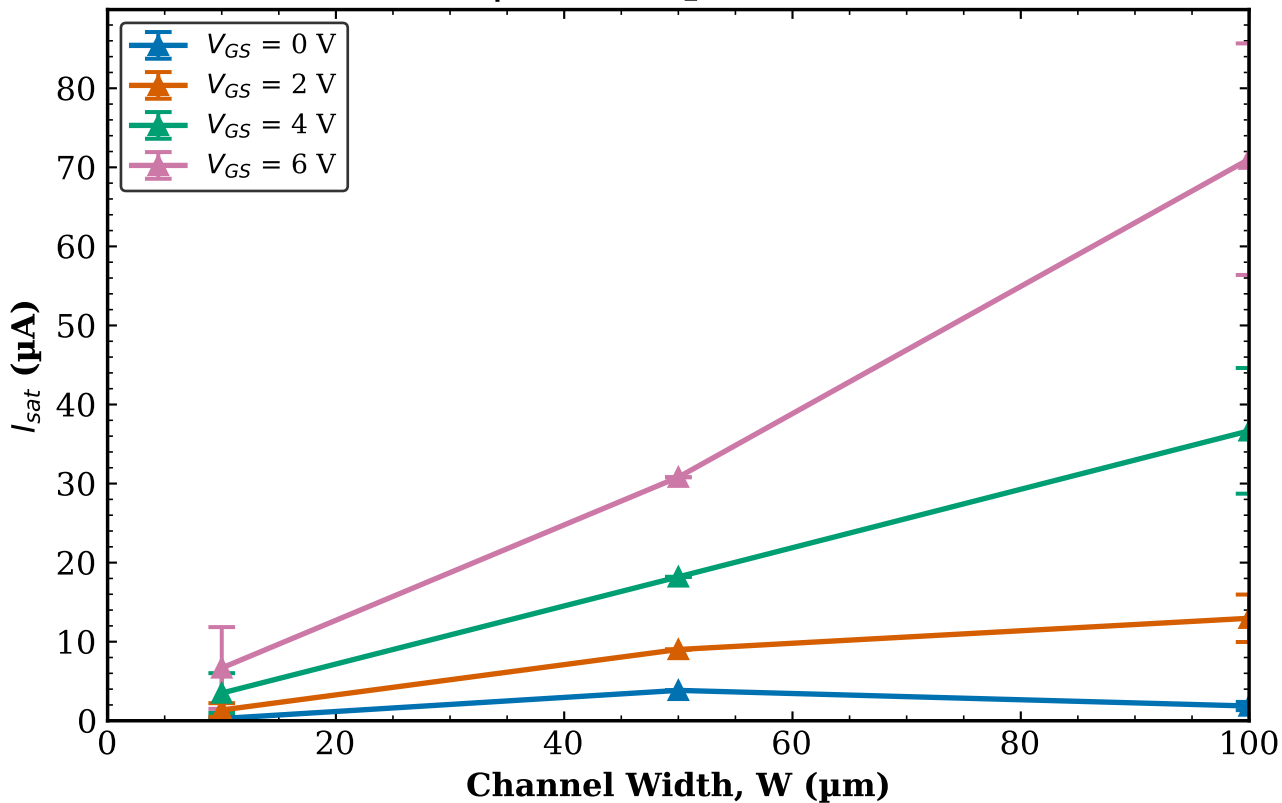
TFT3 Combined (Tr. 1 & 2) I_{sat} vs W | L = 10\text{ }\mu\text{m} (mean \pm std)
